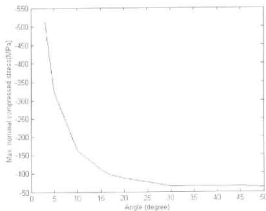
Fig. 3 Variations of the maximum nominal compressed stress with angle \theta from [001] direction for single-slip kink band ( m=0.04 )
